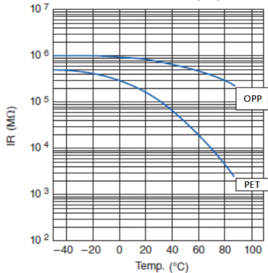
Insulation resistance (MΩ)
